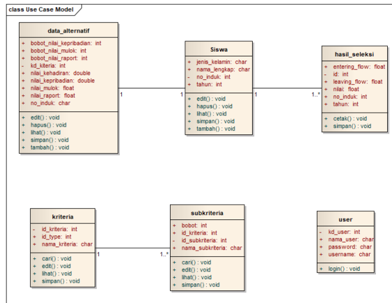
Gambar 3 Class Diagram
